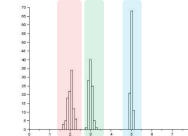
(b) Histogram of estimated gains corresponding to the concentrations
