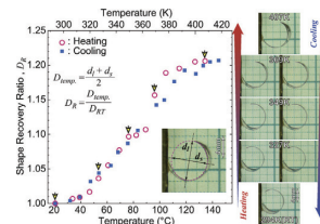
Fig.: Shape recovery ratio versus temperature curves and corresponding shape changes observed during thermal cycle of a TiNi/polyimide single-beam cantilever. The cantilever was activated with a heating heater. It is clear that the film deposited on a polyimide sheet shows two-way motion by thermal cycle. The two-way motion appears to be originated in martensitic and its reverse transformations.
