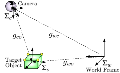
Fig. 1. Eye-in-hand visual feedback systems.
