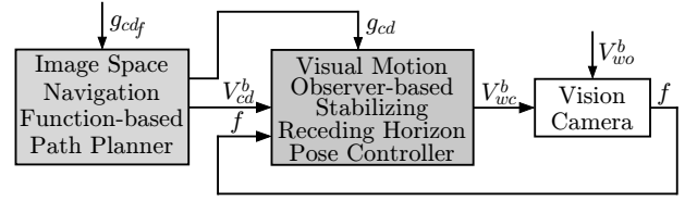
Fig. 3. Block diagram of visual motion stabilizing receding horizon control with image space navigation function-based path planner.
