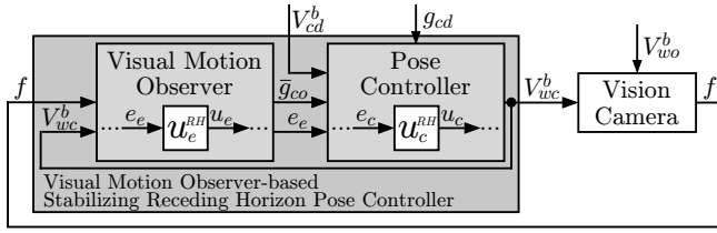
Fig. 2. Block diagram of visual motion stabilizing receding horizon control.
