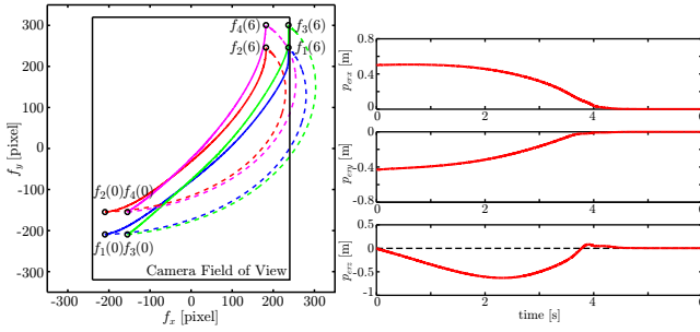
Fig. 4. Trajectory of image feature points f_{co} : Solid; with proposed method: Dashed; with previous one.
